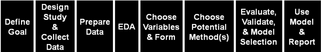
Figure 1: Schematic of the steps in building an empirical model (predictive or explanatory)
